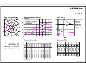
CalcLux Photometrics 4.5 Philips Lighting B.V. Page 1/1
